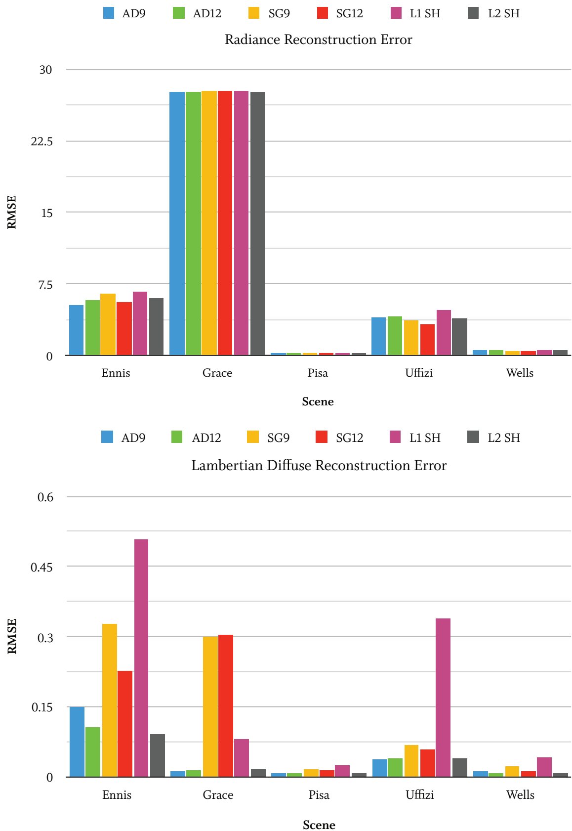
Figure C.6: Comparison graphs of reconstruction error for spherical harmonics, spherical Gaussians, and cosine-lobe Ambient Dice
