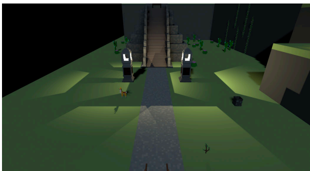
Figure 6.3: Irradiance Caching
